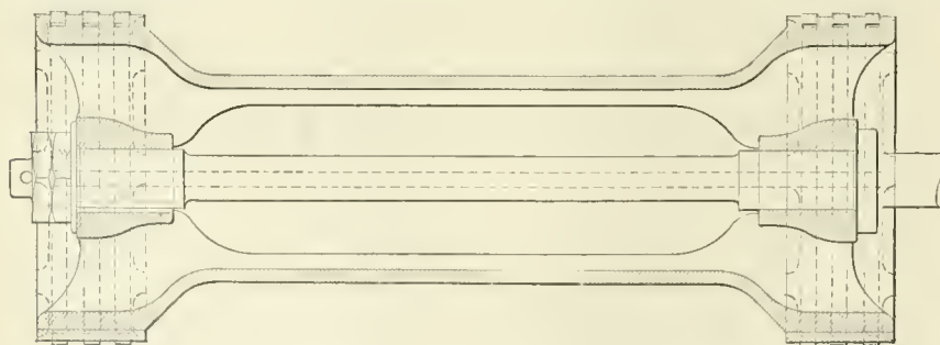
PISTON VALVE, BALDWIN ENGINE. SIX PACKING RINGS.
